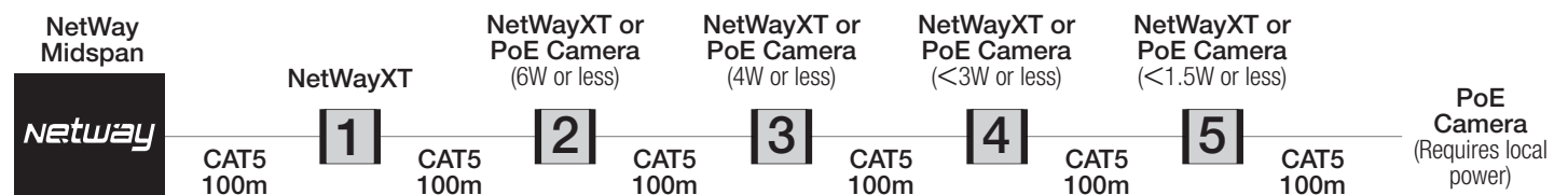
Fig. 5 - Connecting several NetWayXTs on a single port
