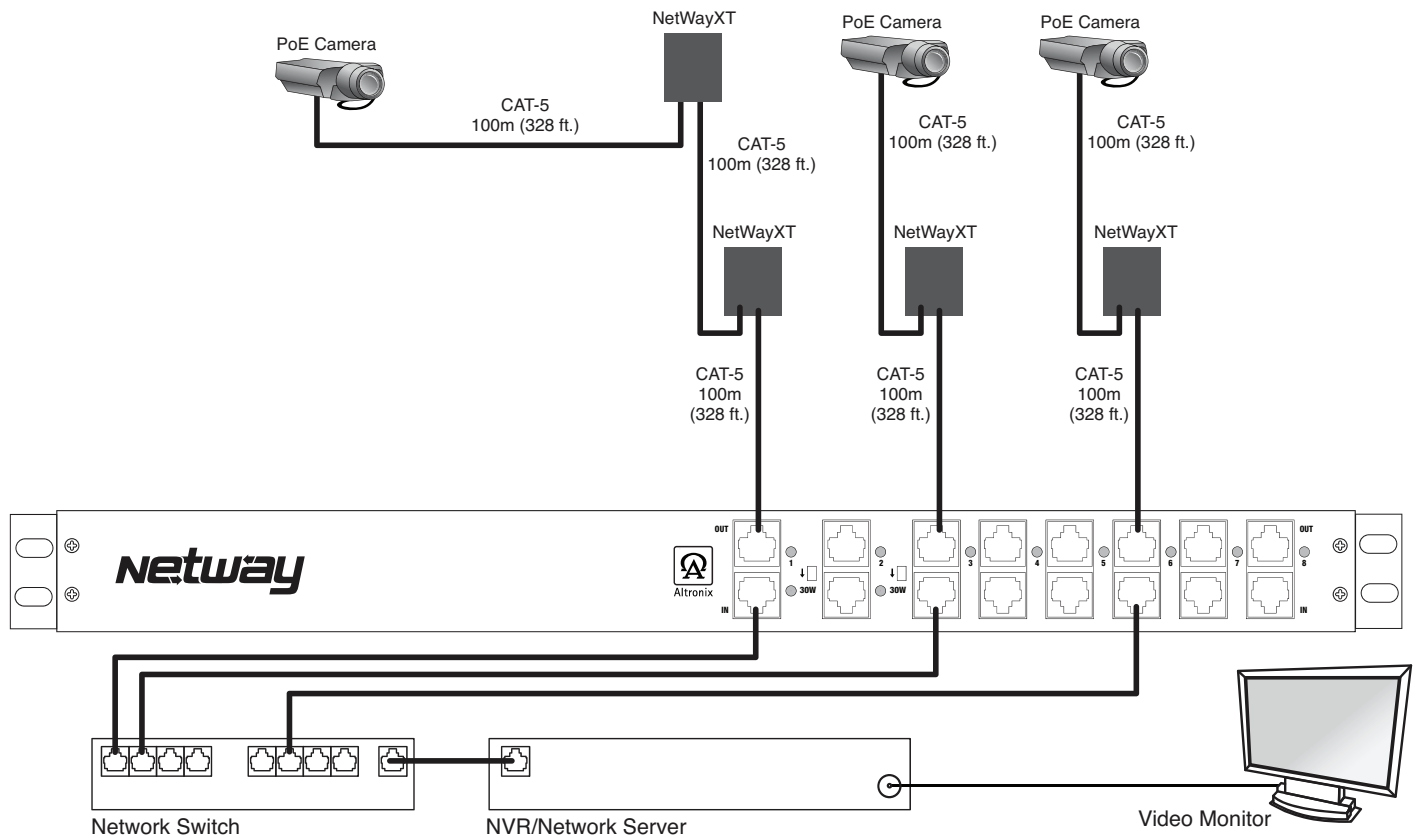
Fig. 5 - Connecting several NetWayXTs on a single port
