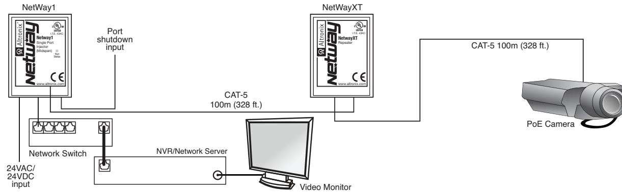
Fig. 3 - NetWayXT connected to NetWay1 Single Port Midspan Injector
