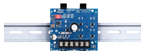
Board mounted on DIN Rail with CLIP4 (front view)
