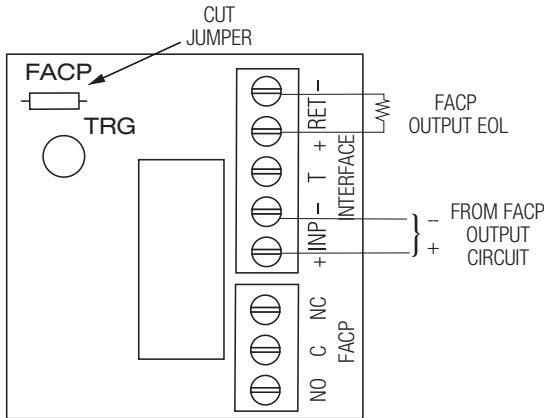
Fig. 5 Normally Open: Non-Latching FACP trigger input:
