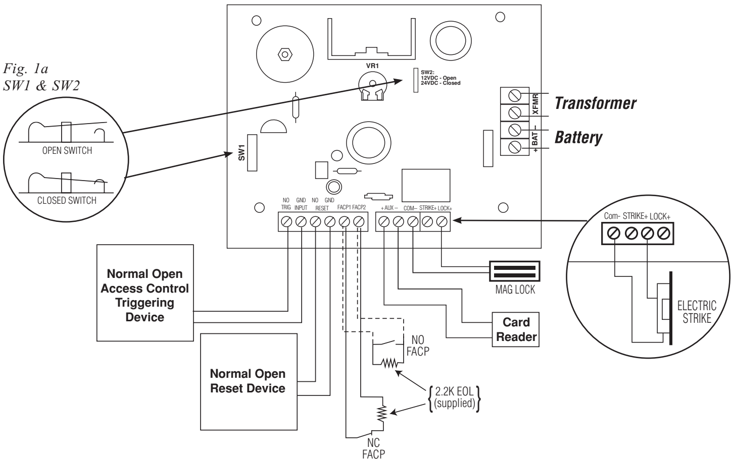
Fig. 1 - Application Diagram:
