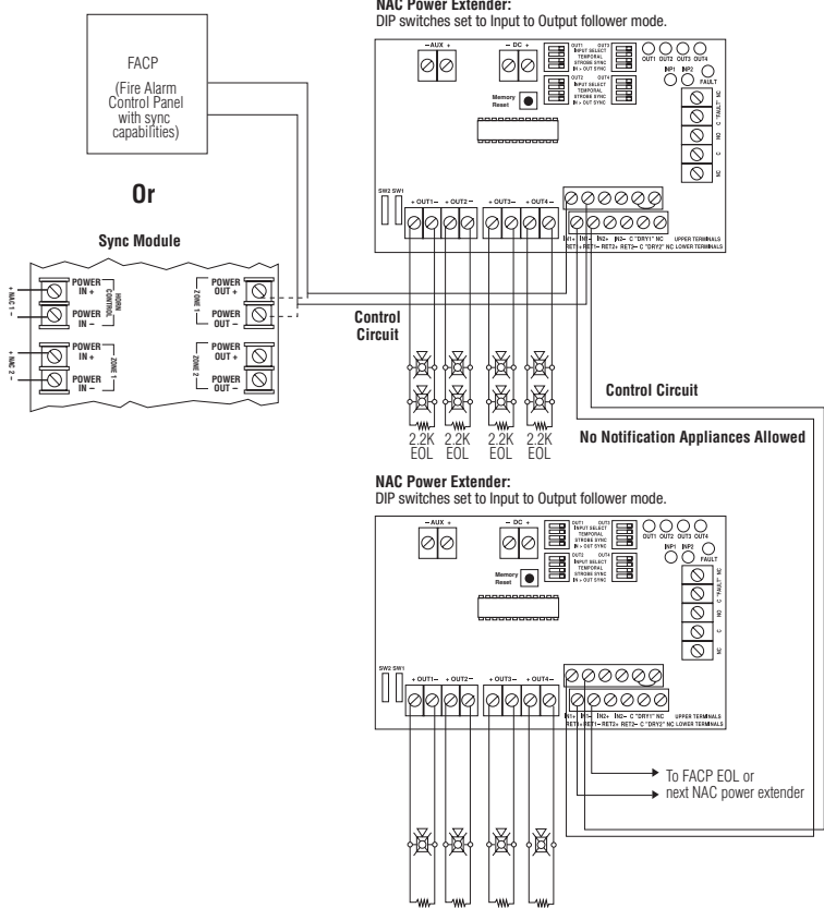
FACP with Sync Output
