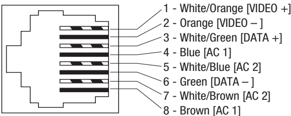
Fig. 3 - CAT-5 Structured Cable Wiring Color Codes and PIN Configurations PVD1-4 on HubSat4DV and Video Balun/Combiner
