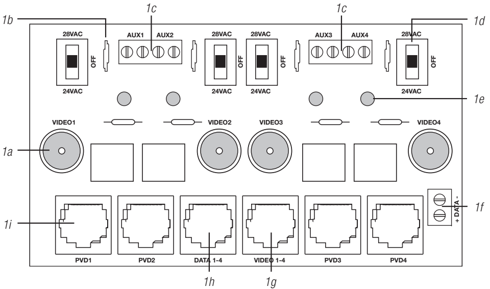
Fig. 1 - HubSat4DV Circuit Board
