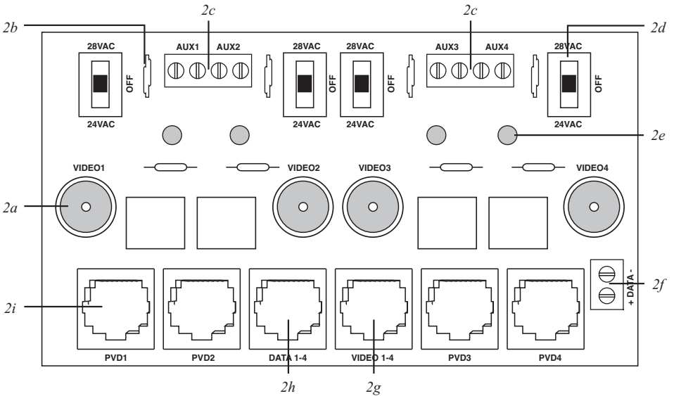
Fig. 2 - HubSat Circuit Board
