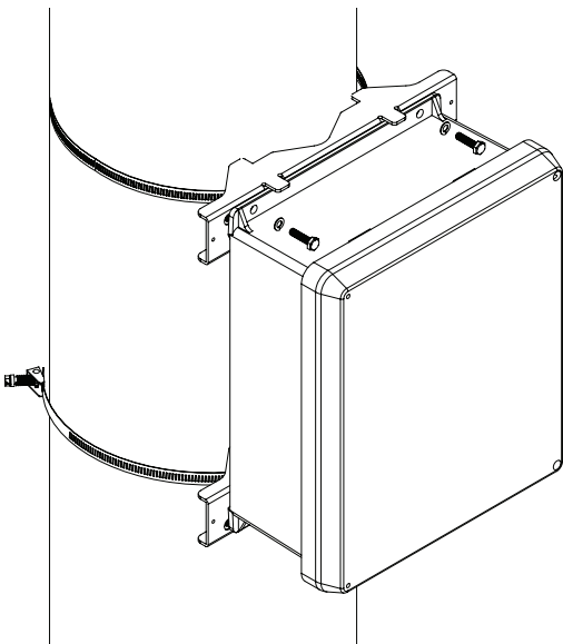
Fig. 9d - 2" to 8" (50.8mm to 203.2mm) diameter round pole
