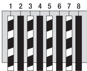
Fig. 3 - CAT-5 Structured Cable Wiring Color Codes
