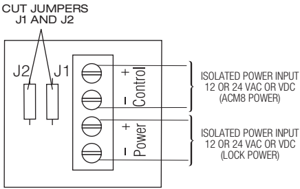
Fig. 10 Optional hook-up using two (2) isolated power supply inputs (Only applicable on Maximal11DV):
