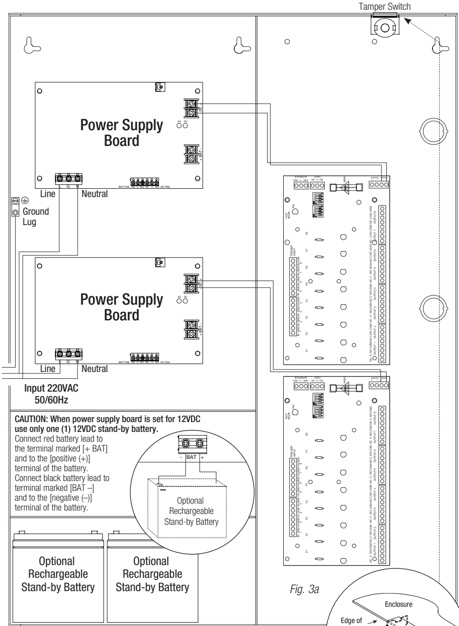
Fig. 3 - Maximal11DV, Maximal33DV, Maximal55DV
