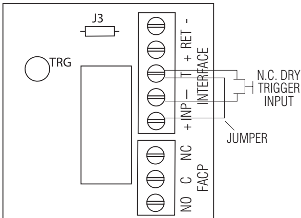
Fig. 10 Normally Closed - Non-Latching FACP trigger input:
