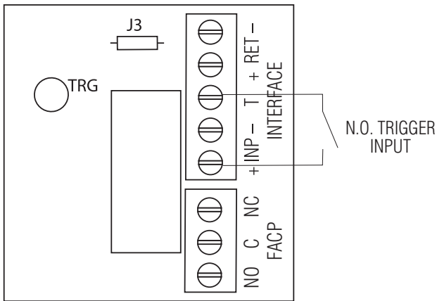
Fig. 8 Normally Open - Non-Latching FACP trigger input:
