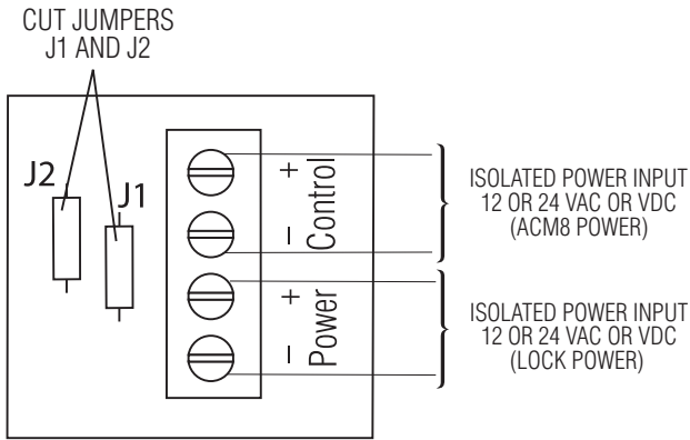
Fig. 6 Optional hook-up using two (2) isolated power supply inputs (Only applicable on Maximal11V):
