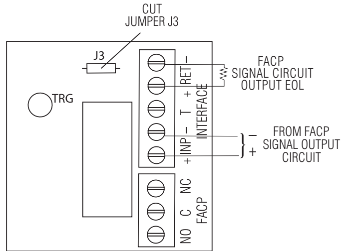
Fig. 9 Normally Open FACP Latching trigger input with reset:
