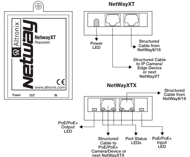
Fig. 4 - NetWayXT/NetWayXTX
