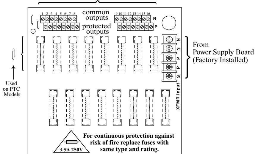
Fig. 5 DC Output to devices 1P-16P Power Outputs, 1N-16N Common Outputs
