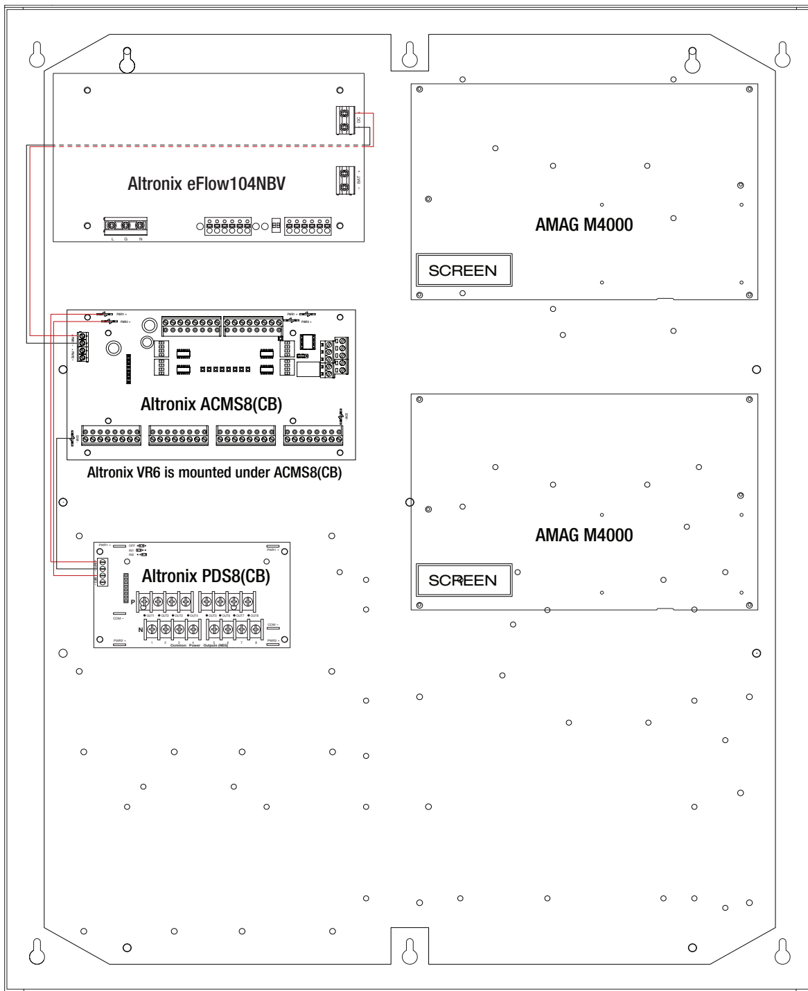
Fig. 3 - T2AGK7F8S(D)V Configuration
