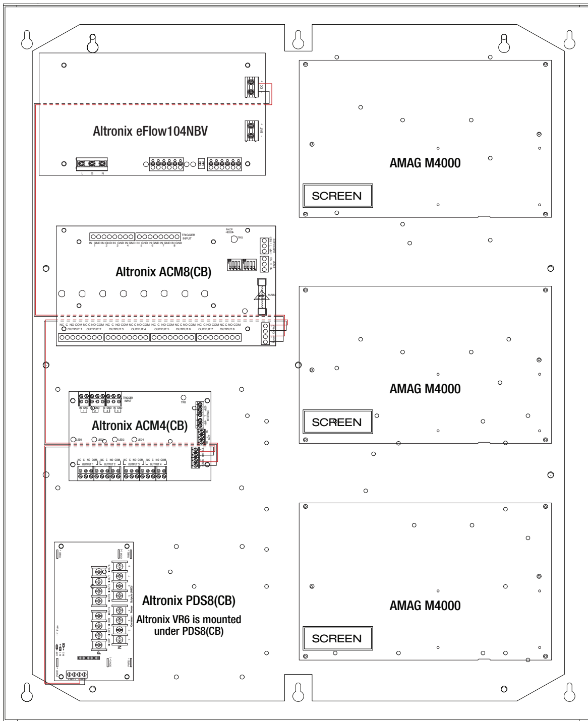
Fig. 4 - T2AGK7F12(D)V Configuration
