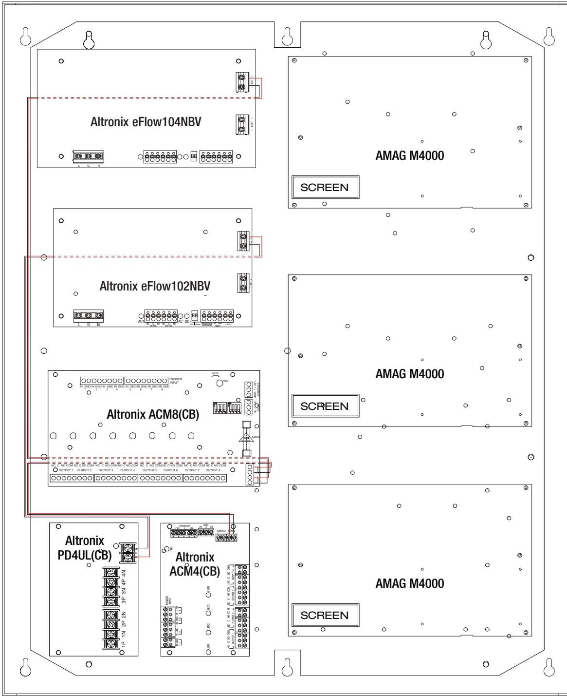
Fig. 6 - T2AGK75F12(D)V Configuration
