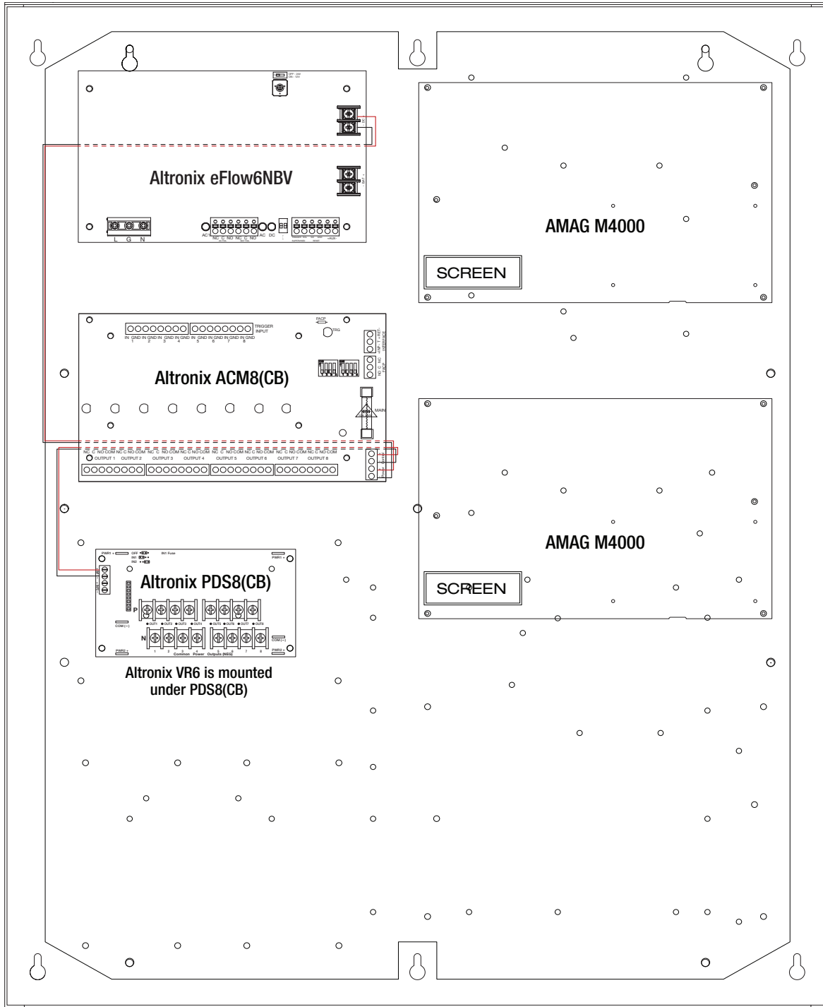
Fig. 2 - T2AGK3F8(D)V Configuration
