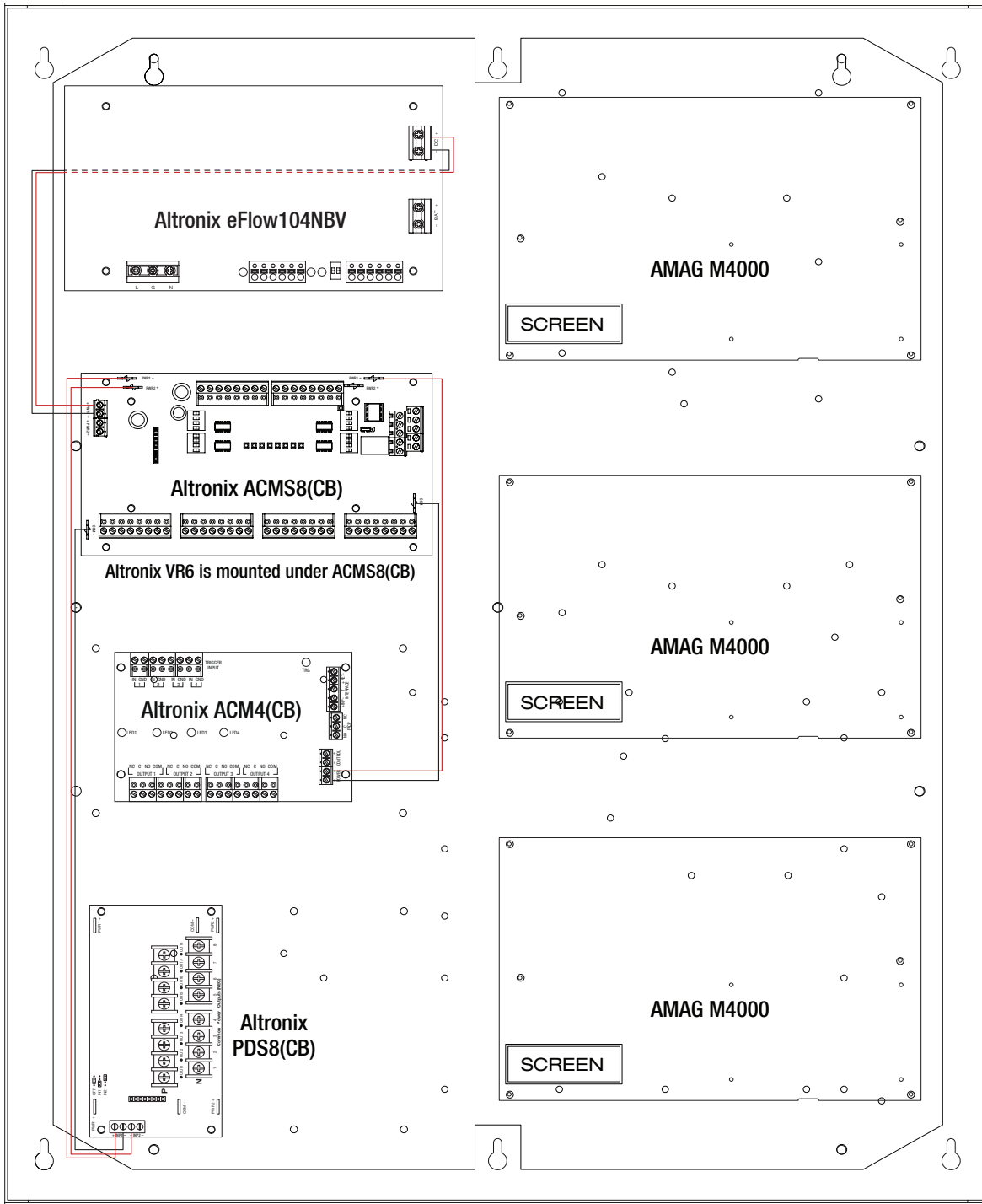
Fig. 5 - T2AGK7F12S(D)V Configuration
