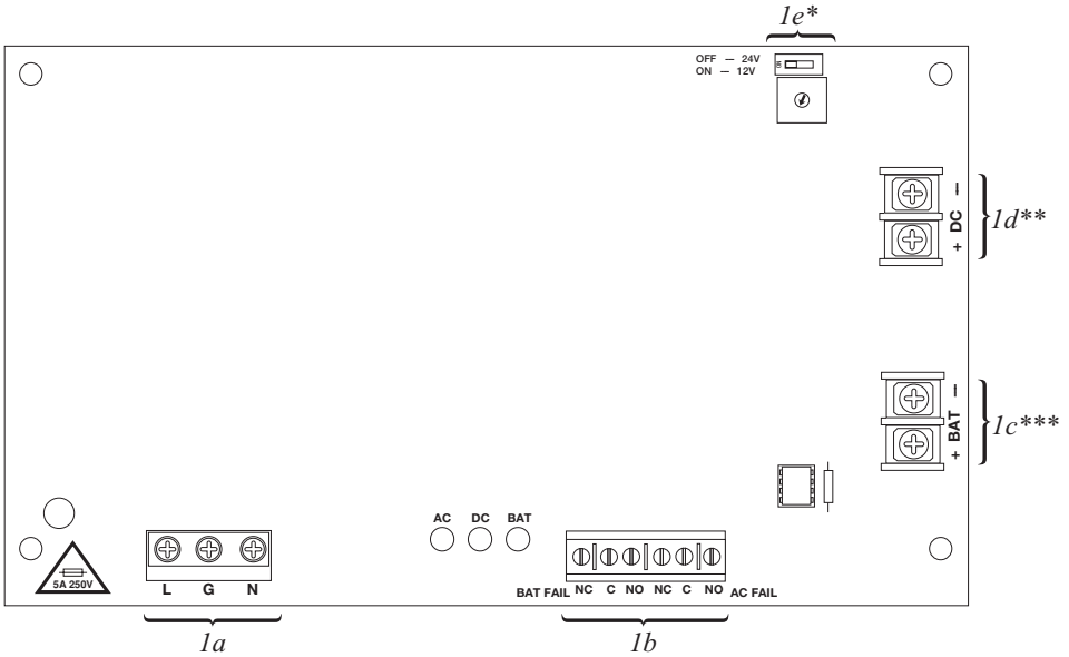
Fig. 1 - ULXB configuration
