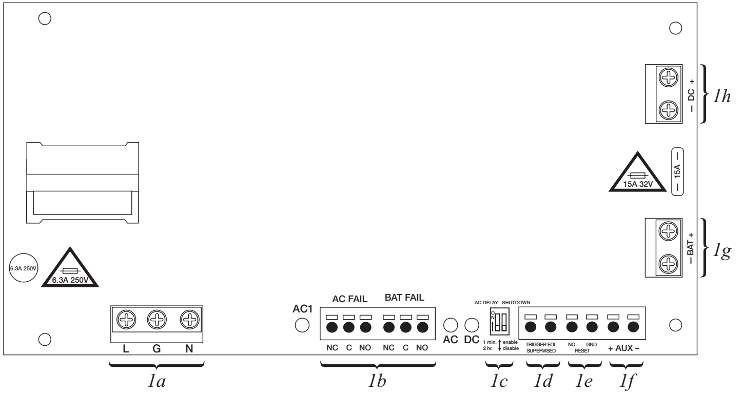
Fig. 1 - eFlow104NBV configuration
