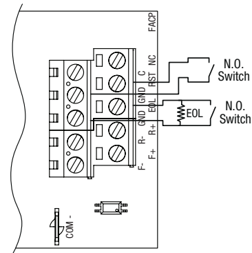
Fig. 14 - Normally Open trigger input (Latching).
