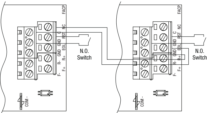
Fig. 8 - Daisy chaining one or more LINQ8ACM(CB) units.
