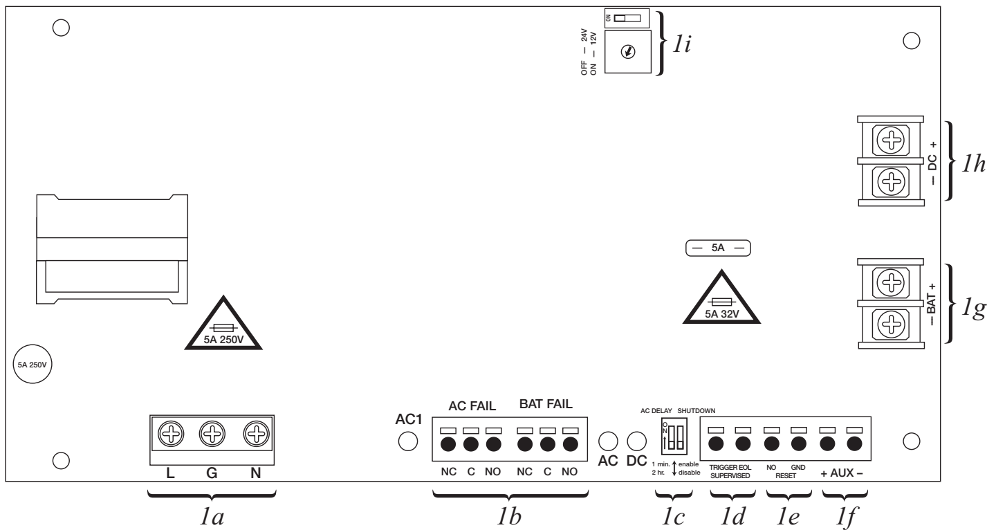
Fig. 1 - eFlow4NB configuration
