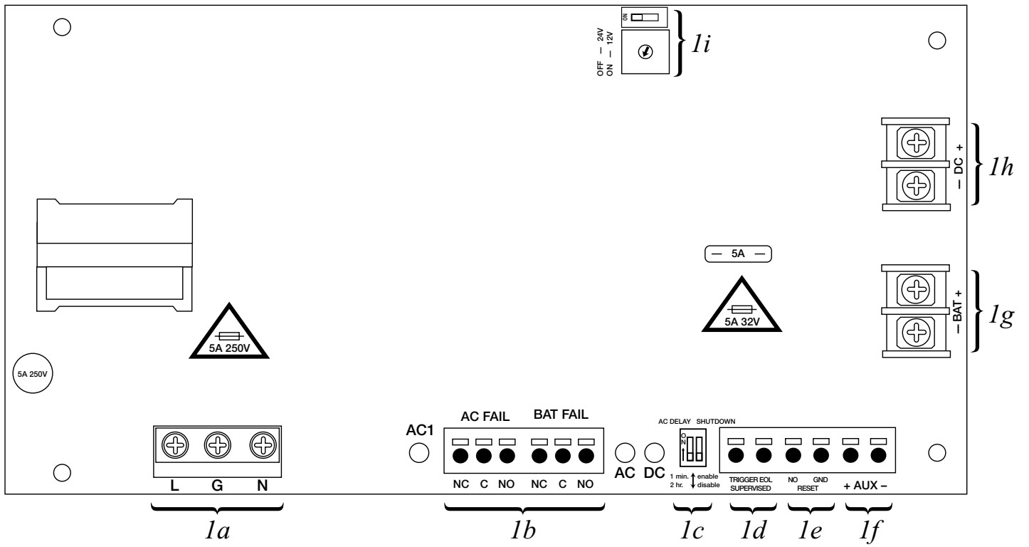
Fig. 1 - eFlow4NBV configuration
