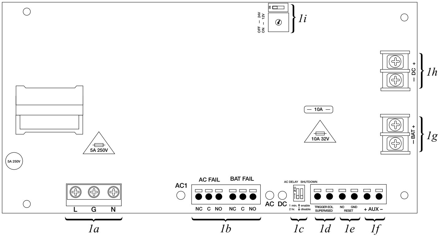
Fig. 1 - eFlow6NBV configuration
