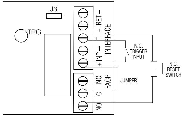
Fig. 8 Normally Open FACP Latching trigger input with reset: (This output has not been evaluated by UL)
