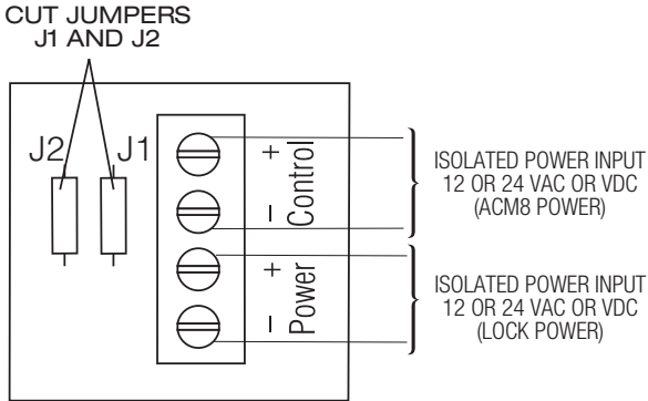
Fig. 5 Optional hook-up using two (2) isolated power supply inputs (Only applicable on eFlow4NA8V):
